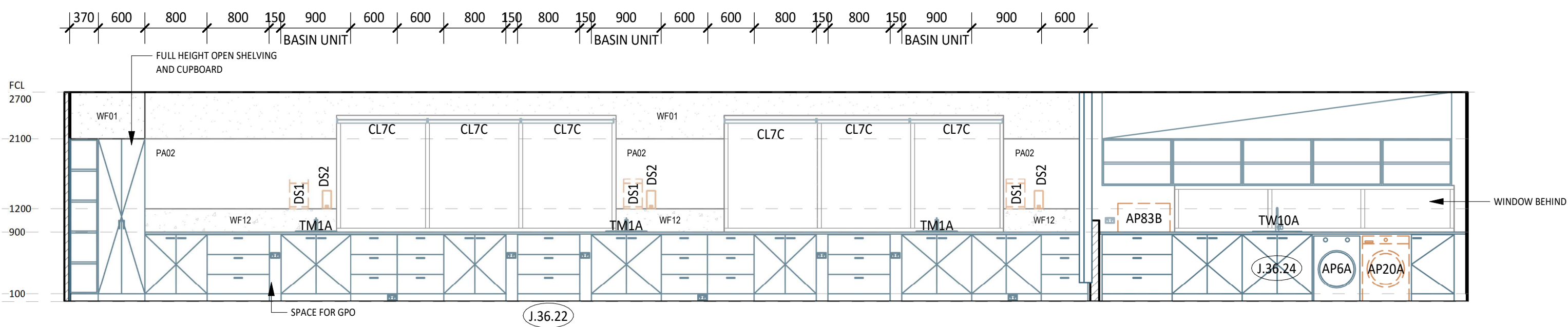
4 ELEVATION DETAIL 1 : 50
