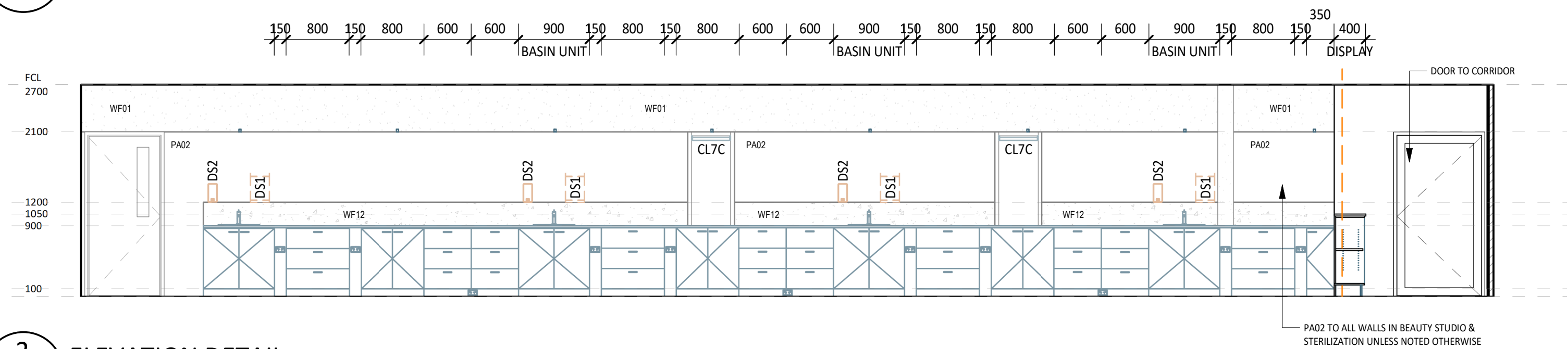
3 ELEVATION DETAIL 1 : 50
